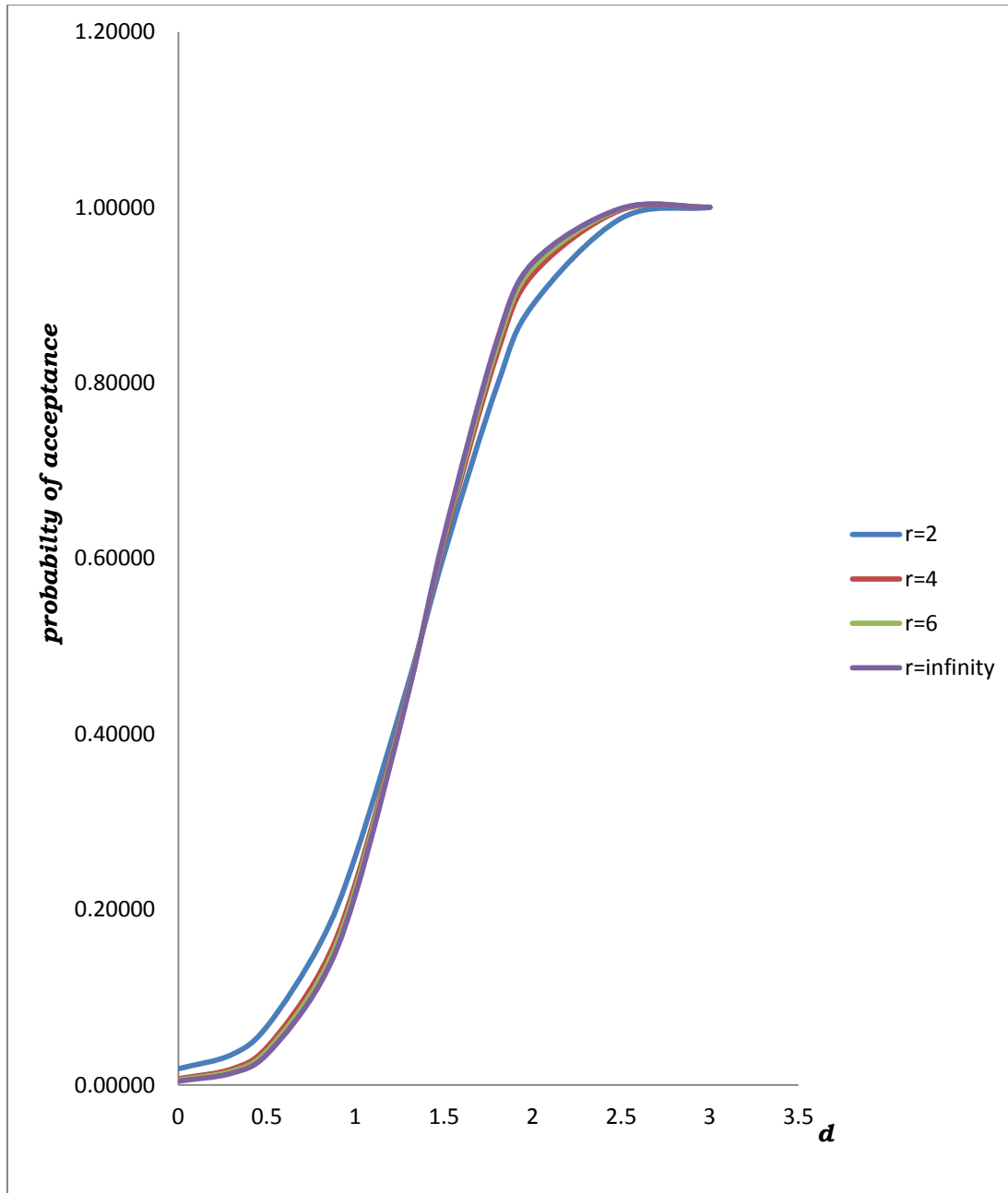
Fig-5: Power curve of average control chart when (\lambda_3, \lambda_3) = (-0.5, -0.5)
