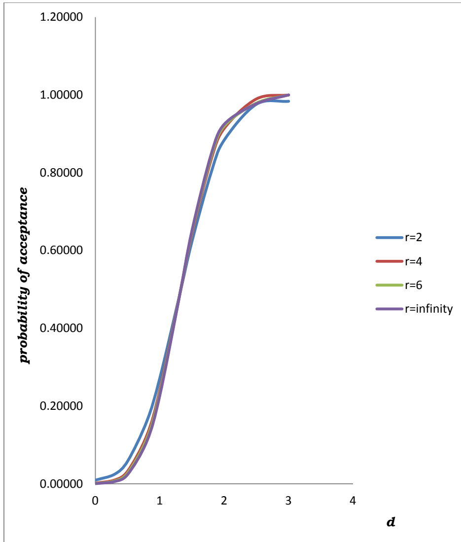
Fig-2: Power curve of average control chart when (\lambda_3, \lambda_3) = (0.5, 0) .
