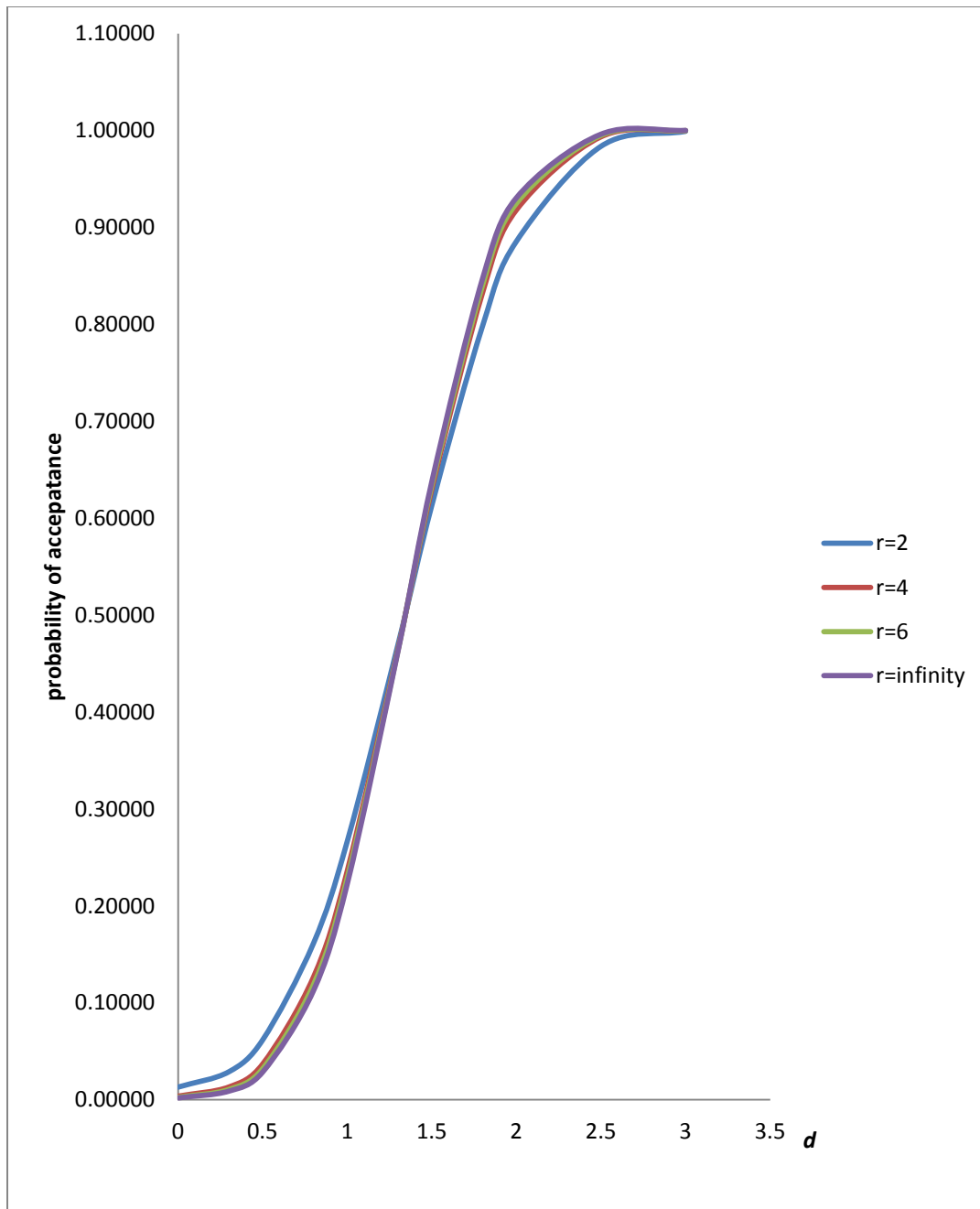
Fig-3: Power curve of average control chart when (\lambda_3, \lambda_3) = (0, -0.5)
