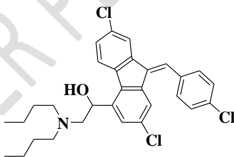
Fig. 1: Chemical structure of lumefantrine
