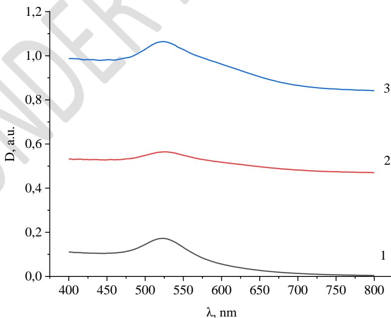
Figure 6. Absorption spectrum of Au nanoparticles stabilized with PEG-200 after 30 days of storage at room temperature
