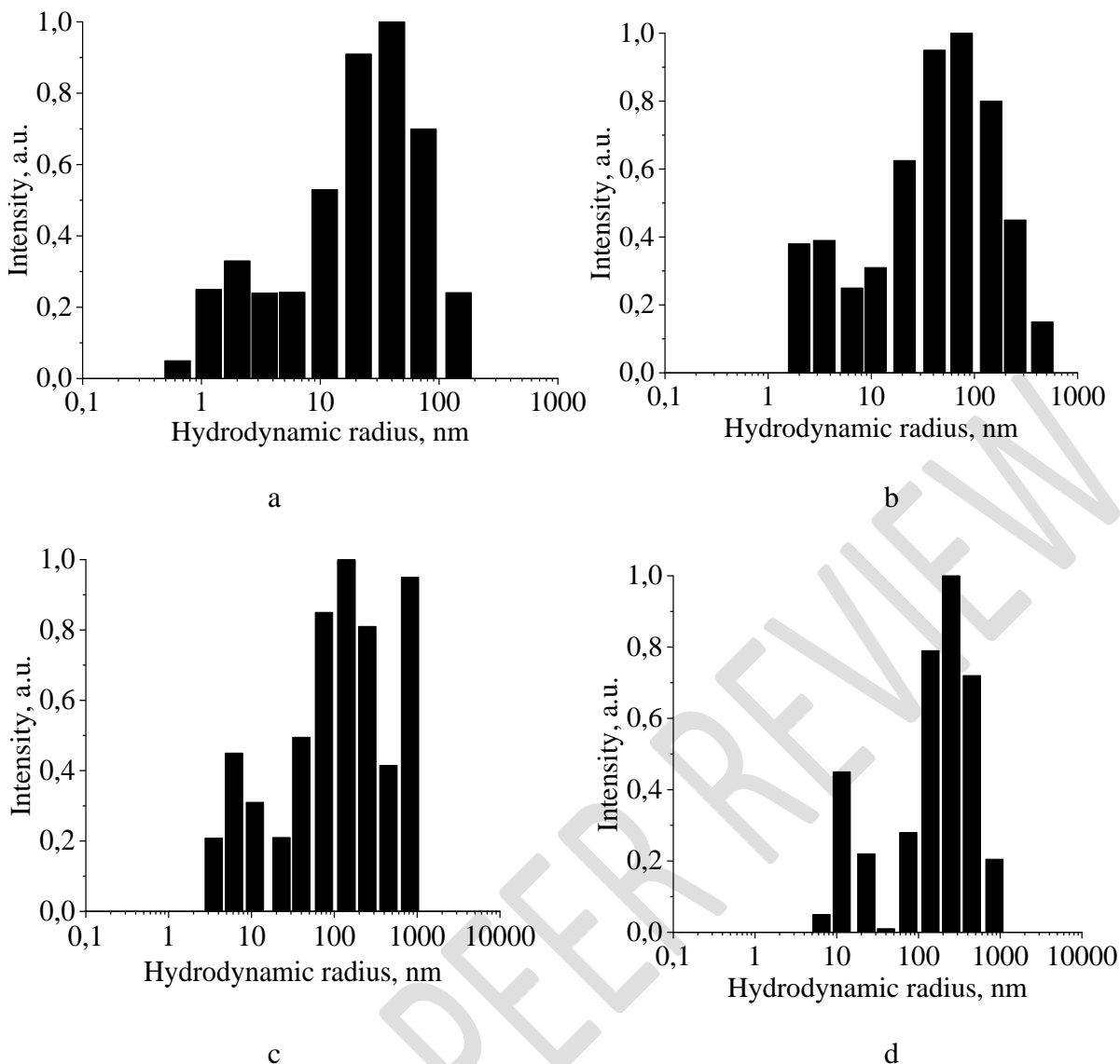
Figure 11. Histograms of the distribution of hydrodynamic radii of Au nanoparticles stabilized with PEG 8000: a-1%; b-5%; c-10%;d-20%
