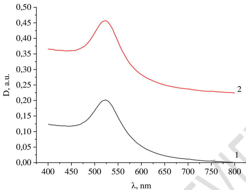
1 – 10 %; 2 – 20 % Figure 9. Absorption spectrum of Au nanoparticles stabilized with PEG-4000 after 30 days of storage at room temperature
