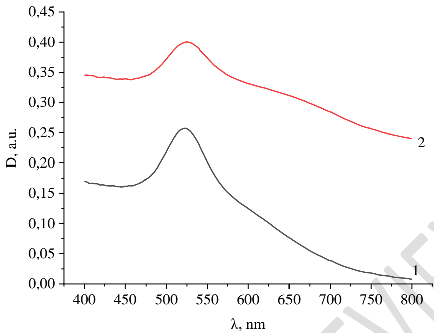
1 – 10 %; 2 – 20 % Figure 7. Absorption spectrum of Au nanoparticles stabilized with PEG-400 after 30 days of storage at room temperature
