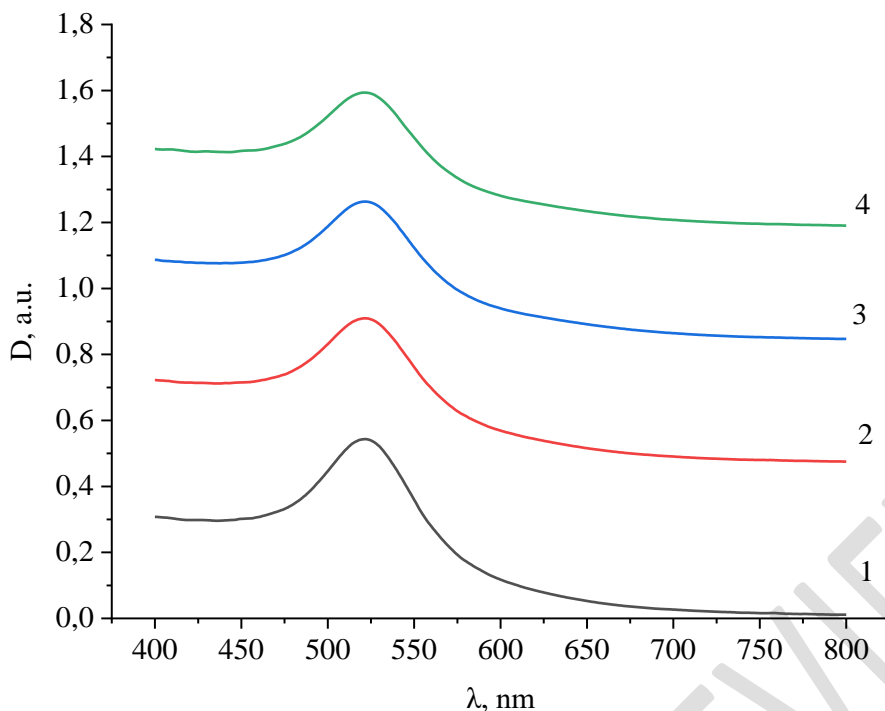
Figure 5. Absorption spectrum of Au nanoparticles stabilized by PEG-6000
